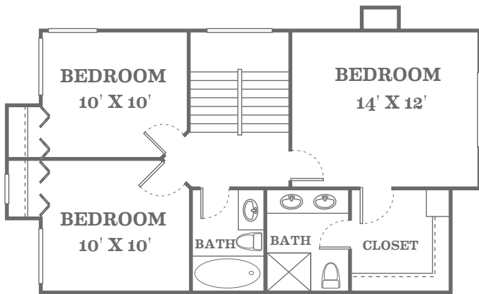
Second Floor
